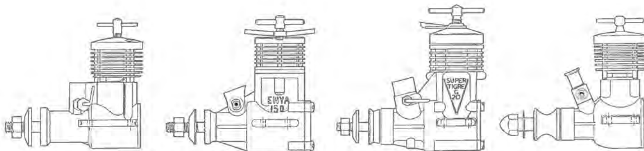
Dieselmotorer: Fra venstre PAW-15D, Enya 15D, Super Tigre G 20, Oliver Tiger MK. II (fra Aeromodeller).
