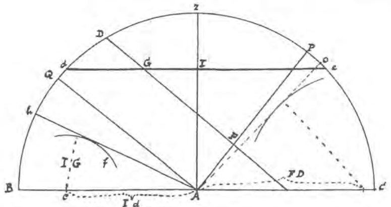
Figur 19. Solens Azimuth.
